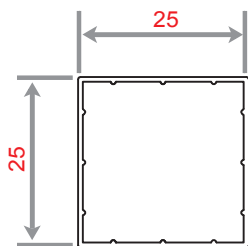
MG 106 WEIGHT 300 KG/M
