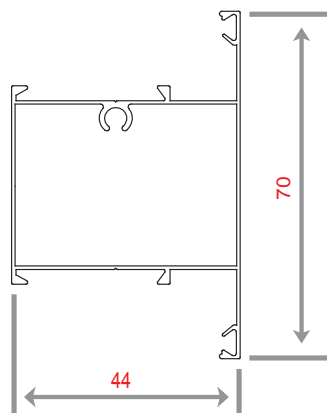
NC 1435 WEIGHT 650 KG/M
