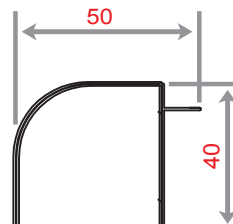
MG 121 WEIGHT 425 KG/M
