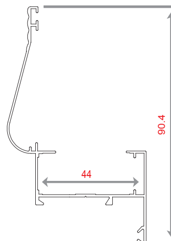
NC 1479/A WEIGHT 669.9 KG/M
