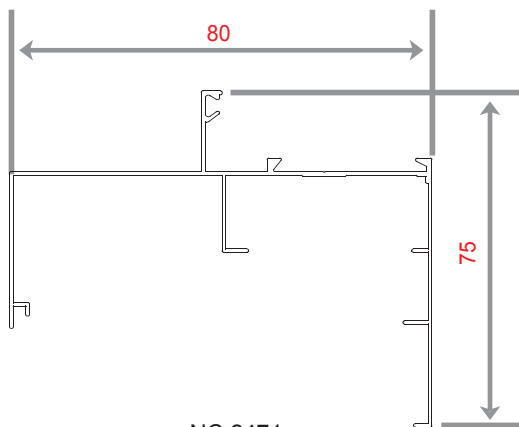
NC 2471 WEIGHT 850 KG/M
