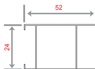
NC 1221 WEIGHT 450 KG/M
