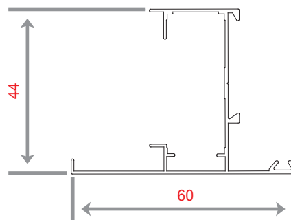
NC 1370 WEIGHT 454.3 KG/M
