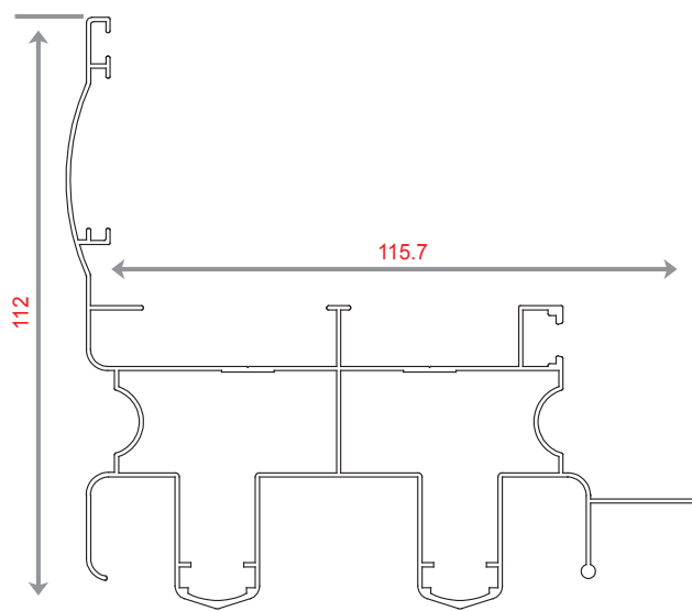
PS 9642 WEIGHT 1696.42 .KG/M
