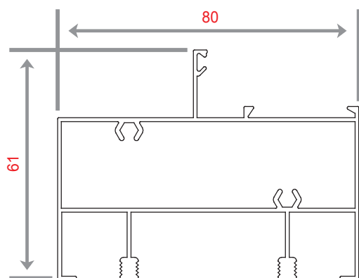
NC 1381 WEIGHT 1289.2 KG/M
