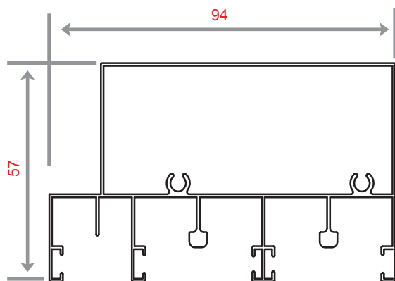
B 616 WEIGHT 1249.2 KG/M
