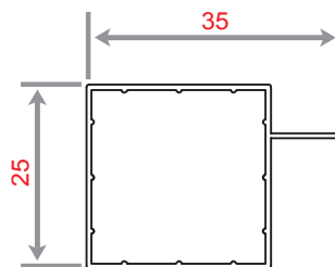
MG 111 WEIGHT 325 KG/M
