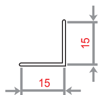
15*15*1 WEIGHT 85.52 KG/M
