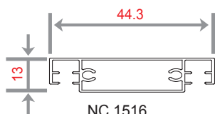
NC 1516 WEIGHT 450 KG/M
