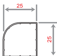
MG 122 WEIGHT 300 KG/M
