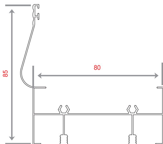
NC 1340/B WEIGHT 903.1 KG/M
