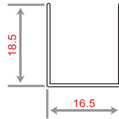
U 613 WEIGHT 140 KG/M
