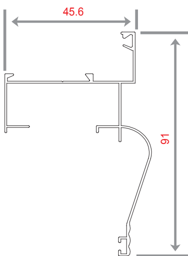
NC 1370-B WEIGHT 600 KG/M
