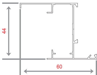
NC 1369 WEIGHT 444.4 KG/M
