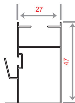
B 703 WEIGHT 446.4 KG/M
