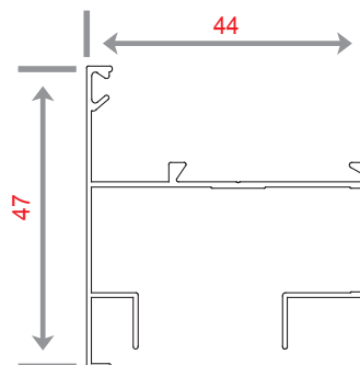
NC 1400 WEIGHT 416.9 KG/M
