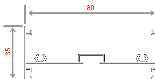
NC 1228 WEIGHT 592.9 KG/M
