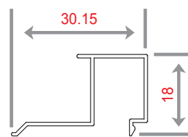
NC 1410 WEIGHT 158.4 KG/M
