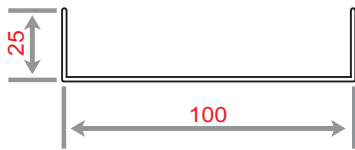
U 100 WEIGHT 743.75 KG/M
