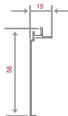
NC 1315 WEIGHT 193.6 KG/M
