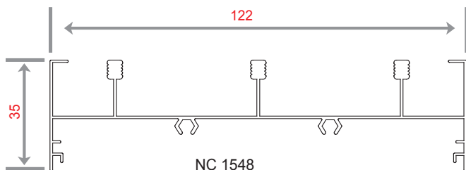
NC 1548 WEIGHT 1200 KG/M
